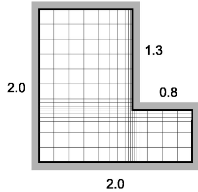
FIG. 11. The L -shaped 2D cavity with a variable grid (schematically).
